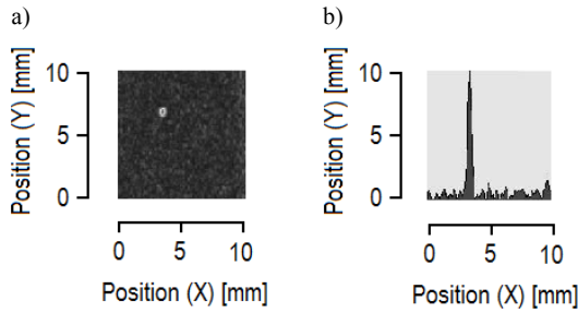
Fig. 10. Laser-ultrasonic 2-D C-scan (a) with an assumed sound depth of 1.5 mm and profile (b).
