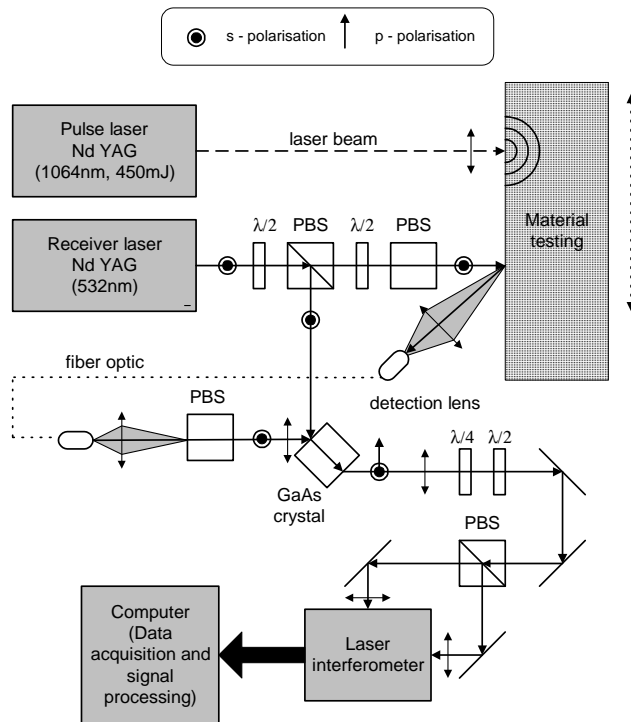
Fig. 5. Laser ultrasonic set-up.
