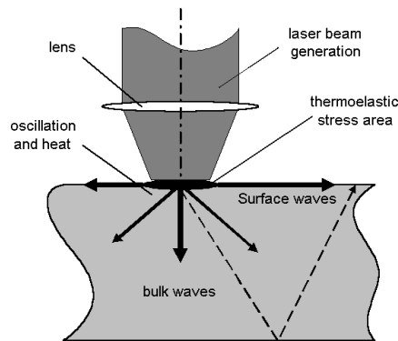
Fig. 6. Non-destructive excitation of different ultrasound waves in a material.
