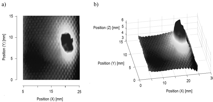
Fig. 7. Example C-scan (20x15 μm) of 35 J impact damage on the material: a) 2-D, b) 3-D.
