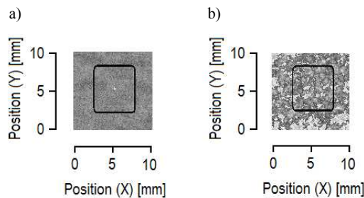
Fig. 12. Laser-ultrasonic 2-D C-scan with assumed sound depth: a) 1.5 mm, b) over 3 mm.
