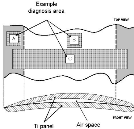
Fig. 8. Simplified intersection of the blade.
