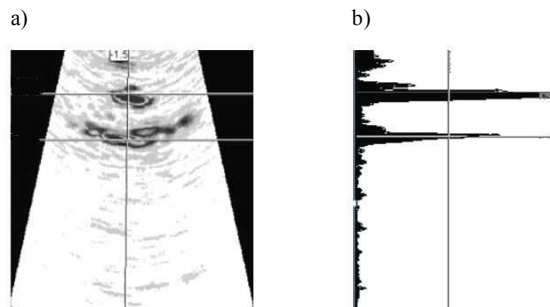
Fig. 4. Example of the ultrasonic image of the analysed blade: a) general view, b) chosen intersection.
