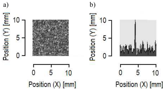
Fig. 11. Laser-ultrasonic 2-D C-scan (a) with assumed sound depth over 3 mm and profile (b).
