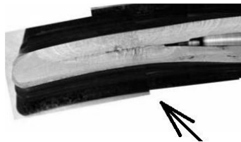
Fig. 3. Examples of damage in the joint of 3 mm-thick composite plates (Rolls-Royce).
